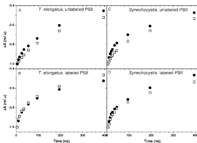
Figure 5. Consequences of the substitution of 3F- Y_Z for Y_Z on the dependence upon temperature of the fast component in the reduction of P_{680}^{++} , at pH 9.2. The left column shows the reduction of P_{680}^{++} in the hundreds of nanoseconds time range in the unlabeled (panel A) and labeled (panel B) PSII core complexes from T. elongatus . The solid circles and open squares show the kinetics at 25–28 and 5 °C, respectively. The right column shows the reduction of P_{680}^{++} in the hundreds of nanoseconds time range in the unlabeled (panel C) and labeled (panel D) PSII core complexes from Synechocystis . The solid circles and open squares depict the kinetics at high and low temperature, respectively. Note that the ordinate axis does not go to 0 and that the figure is a focus on the early events. The fit yielded the following time constants for the fast component: T. elongatus : (panel A, unlabeled) 1.75 \times 10^7 \text{ s}^{-1} \pm 1.7 \times 10^6 at 25 °C and 1.05 \times 10^7 \text{ s}^{-1} \pm 1.8 \times 10^6 at 5 °C; (panel B, labeled) 3.2 \times 10^7 \text{ s}^{-1} \pm 4.2 \times 10^6 at 25 °C and 3.1 \times 10^7 \text{ s}^{-1} \pm 4.5 \times 10^6 at 5 °C; Synechocystis : (panel C, unlabeled) 3.7 \times 10^7 \text{ s}^{-1} \pm 5.7 \times 10^6 at 28 °C and 1.3 \times 10^7 \text{ s}^{-1} \pm 5.8 \times 10^6 at 5 °C; (panel D, labeled) 5.2 \times 10^7 \text{ s}^{-1} \pm 8.2 \times 10^6 at 28 °C and 3.1 \times 10^7 \text{ s}^{-1} \pm 7.5 \times 10^6 at 5 °C.
