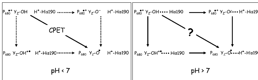
Figure 1. Scheme depicting the reaction pathways for the electron and proton transfer from the phenol group of Y_Z in Mn-depleted PSII. (Left) Situation proposed to prevail at low pH, where the nearby proton-accepting base (shown here as being D_1 -His190, see text for a discussion) is protonated and thus unavailable as a proton acceptor. As discussed in the text, the characteristics of the oxidation rate of Y_Z are those expected for a concerted proton/electron transfer (CPET). (Right) Situation thought to prevail above pH \approx 7 , where a proton-accepting base in close vicinity to the phenol group of Y_Z is available. The nature of the coupling between the electron transfer and proton transfer from the phenol group of Y_Z is the subject of the present study.
