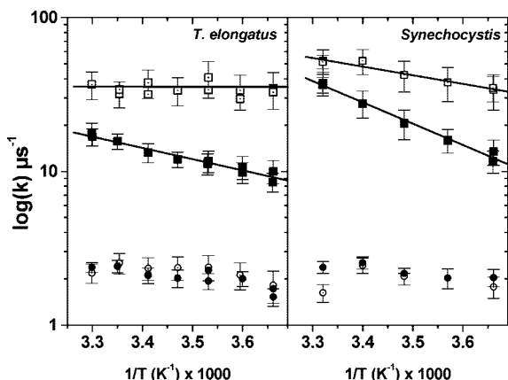
Figure 7. Arrhenius plot of the rates of the first (square) and second component (circle) in the reduction of P_{680}^{++} at pH 9.2, in unlabeled (solid symbols) and labeled (open symbols) PSII complexes from T. elongatus (left panel) and Synechocystis sp. PCC 6803 (right panel). The data were linearly fit to extract the activation energy (the results are shown as the solid lines), and the fit yielded the following values: T. elongatus : 120 \pm 30 meV (unlabeled PSII), 0 \pm 25 meV (labeled PSII); Synechocystis : 220 \pm 35 meV (unlabeled PSII) and 110 \pm 25 meV (labeled PSII).
